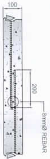
REBAR SPlicing DETAIL SCALE 1 : 12.5 M
